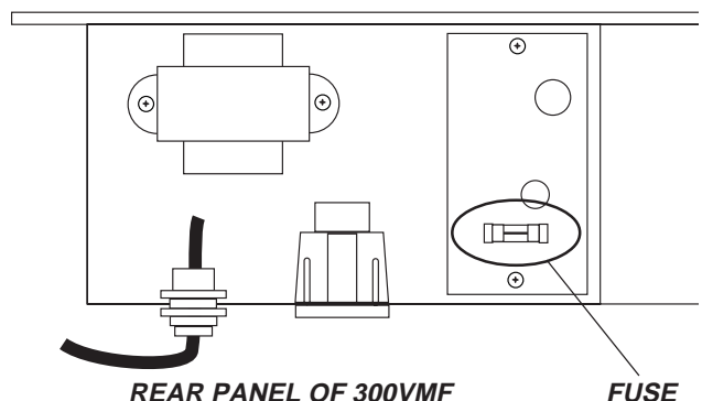
Figure 3 - TOP VIEW OF 300VMF WITH COVER REMOVED SHOWING INTERNAL FUSE LOCATION.
